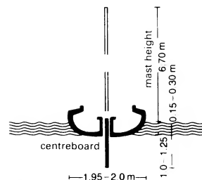
11 Dinghy: section
